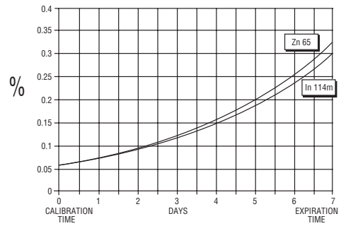
Graph 1 - Radionuclidic Impurities
